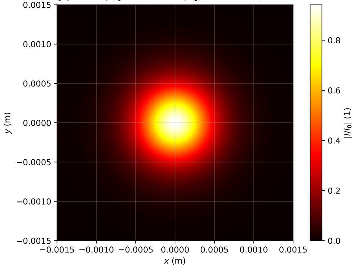
Intensity profile I(x, y, z = 3.662m)/I_0 , P_{in}=0.8P_{cr} , artificial time
